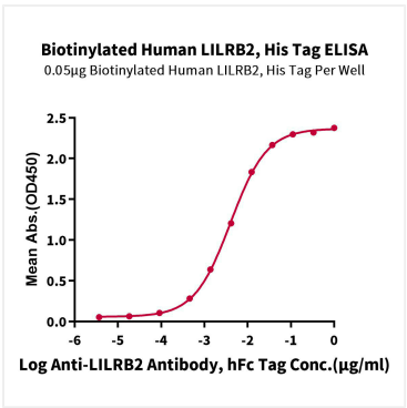
Immobilized Biotinylated Human LILRB2, His Tag at 0.5 µg/mL (100 µL/Well) on streptavidin (5 µg/mL) precoated plate. Dose response curve for Anti-LILRB2 Antibody, hFc Tag with the EC 50 of 4.0ng/mL determined by ELISA.
