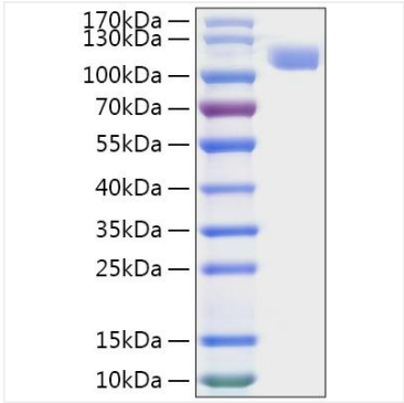
Recombinant MERS-CoV Spike S1 Protein was determined by SDS-PAGE under reducing conditions with Coomassie Blue.
