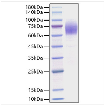
Recombinant Mouse Thrombopoietin/THPO Protein was determined by SDS-PAGE under reducing conditions with Coomassie Blue.
