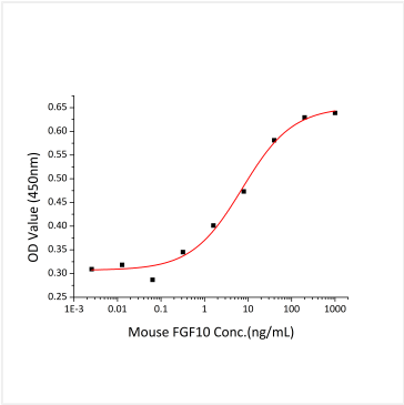
Measured in a cell proliferation assay using 4MBr-5 rhesus monkey epithelial cells. The ED 50 for this effect is 3.66-14.64 ng/mL, corresponding to a specific activity of 56.83×10 4 ~2.73×10 5 units/mg.
