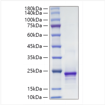
Recombinant Mouse FGF-10 Protein was determined by SDS-PAGE under reducing conditions with Coomassie Blue.
