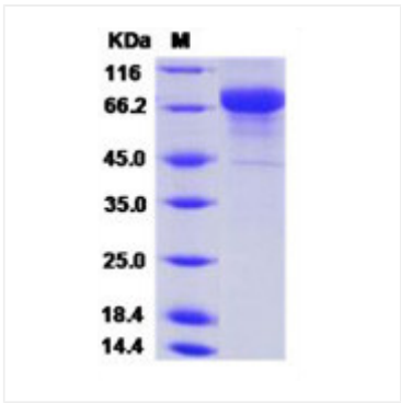
Recombinant Influenza A H3N2 (A/Wisconsin/67/2005) Hemagglutinin/HA Protein was determined by SDS-PAGE under reducing conditions with Coomassie Blue.
