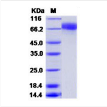
Recombinant Influenza A H3N2 (A/Texas/50/2012) Hemagglutinin/HA Protein was determined by SDS-PAGE under reducing conditions with Coomassie Blue.
